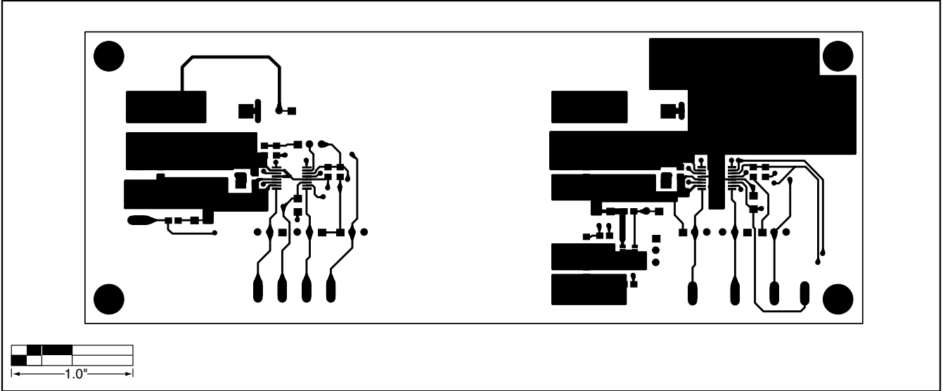
Figure 5. MAX1763 EV Kit PCB Layout—Component Side
