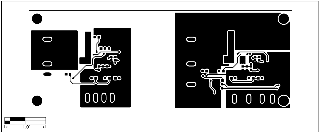
Figure 6. MAX1763 EV Kit PCB Layout—Solder Side
